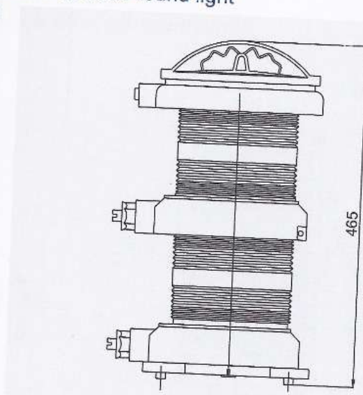
CXH6-101P 双层环照灯 double-deck all-round light
