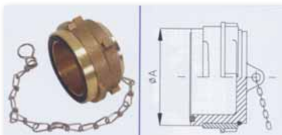
Blank caps with chain, with locking
