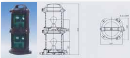
CXH1-10P Full-plastic double-deck starboard light
