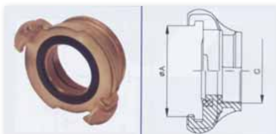
Adapters – female thread
