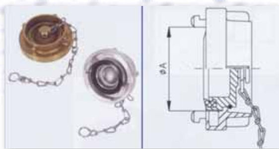
Blank cap with chain
