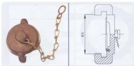
Blank cap with chain
