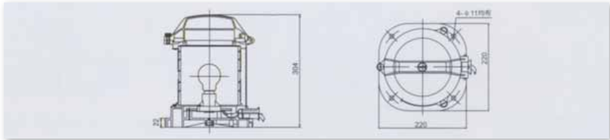
CXH1-1P Full-plastic starboard light
