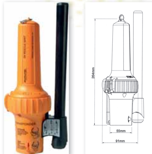
Mc Murdo SART S-4
