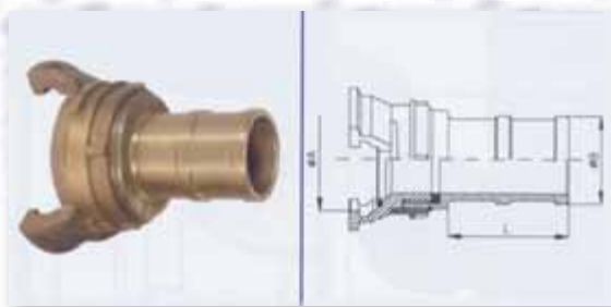
Delivery hose couplings – male/female
