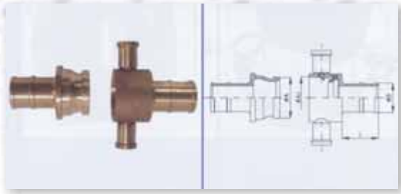
Delivery Hose Couplings – male/female
