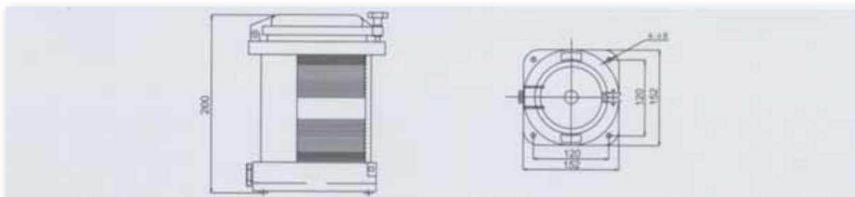
CXH1-21P Starboard light
