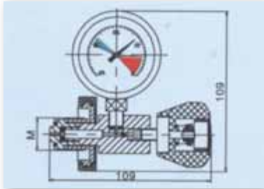
Pressure gauge unit
