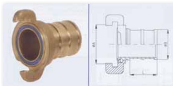
Delivery hose couplings
