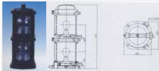
CXH4-10P Full-plastic double-deck stern light
